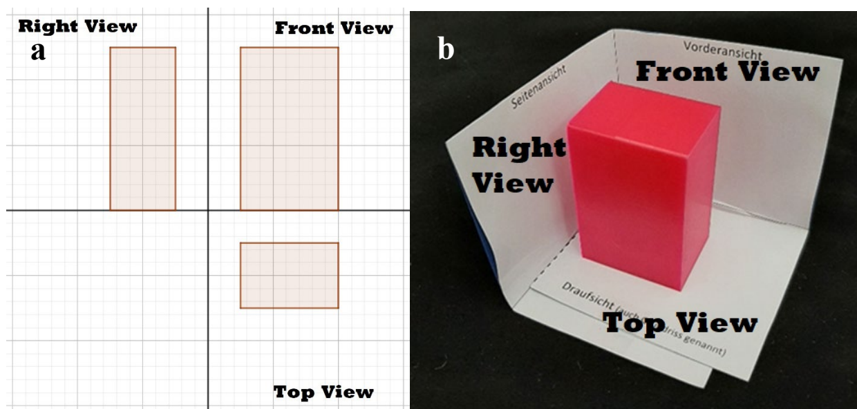
Figure 1: Planes of a multiview projection (a) and a three-dimensional object in a coordinate corner (b)
